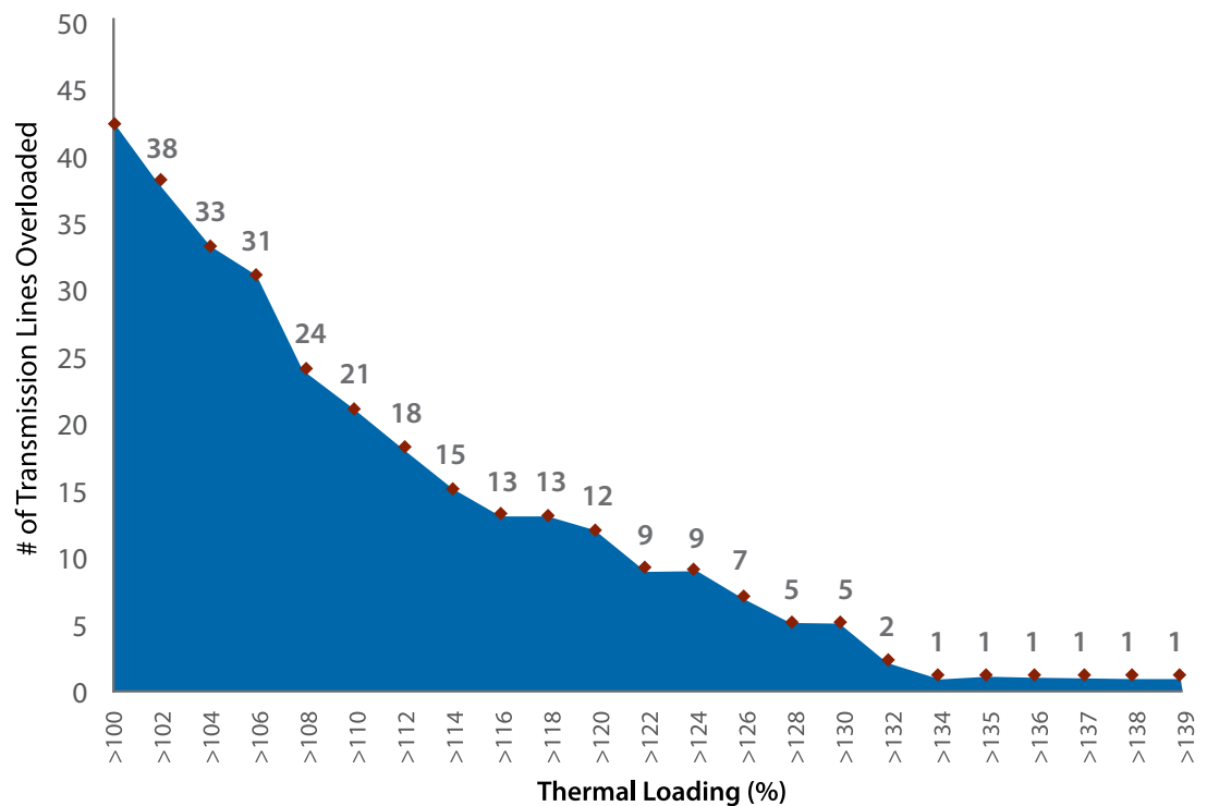
MISO Incremental Transmission Line Overloads Under Proposed CPP
